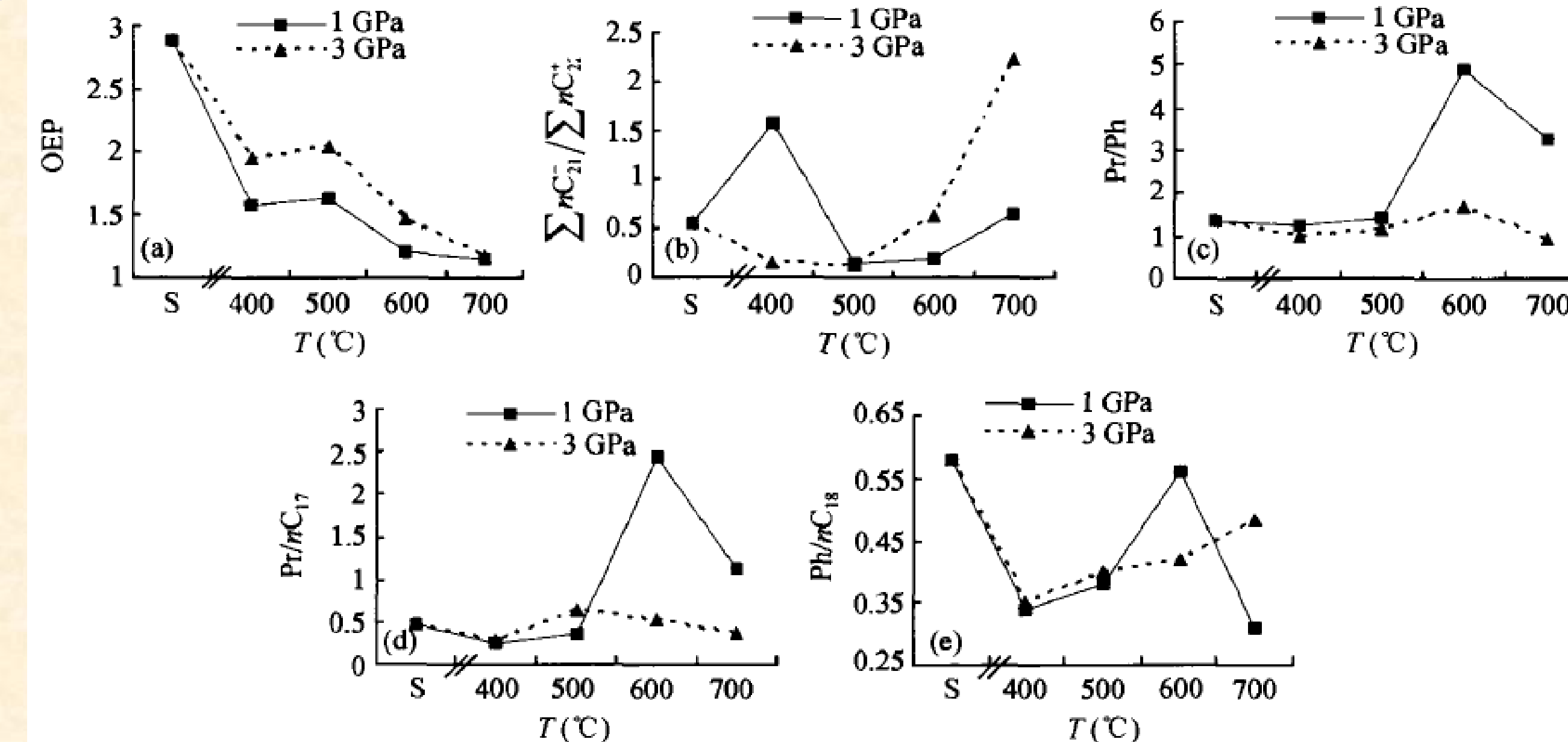
Fig.7 Variations of n -alkane parameters with temperature and pressure (Wang et al., 2006)
