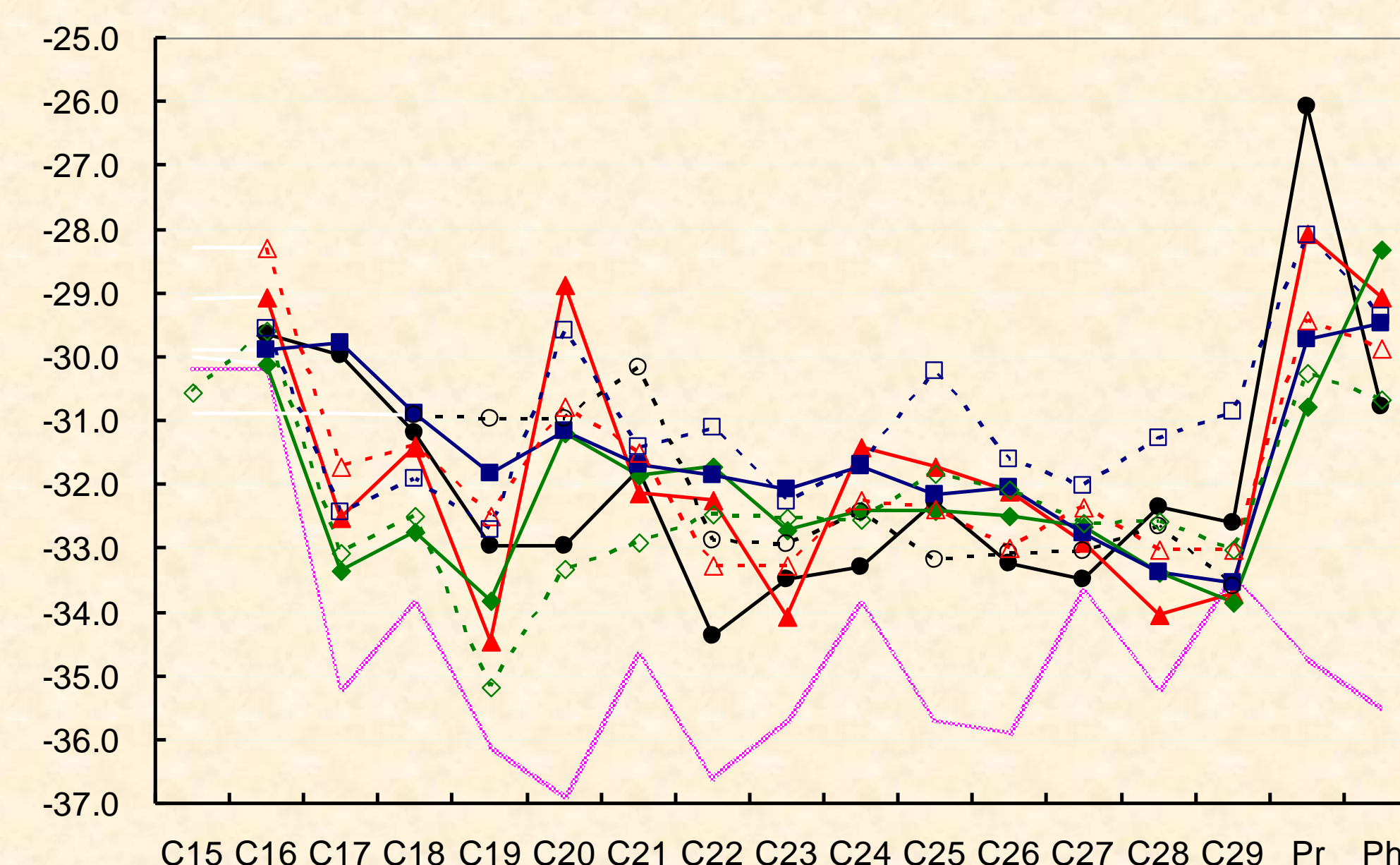
Fig.8 Carbon isotopic profiles of n -alkanes from the lignite and pyrolysates at 3 GPa and different temperatures
